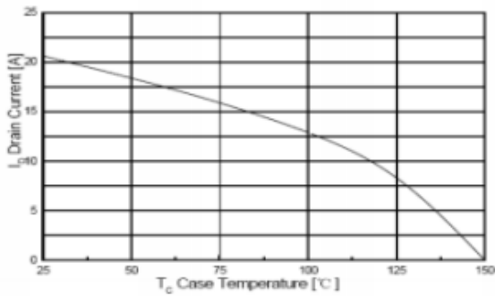
Maximum Drain Current vs. Case Temperature
