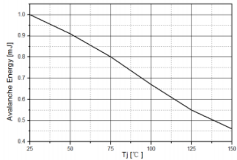
Single Pulsed Avalanche Energy Variation vs. Temperature
