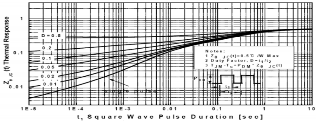
Transient Thermal Response Curve For TO-220F
