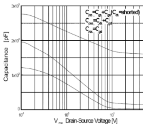
Capacitance Characteristics
