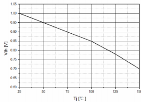
Gate Threshold Voltage Variation vs. Temperature
