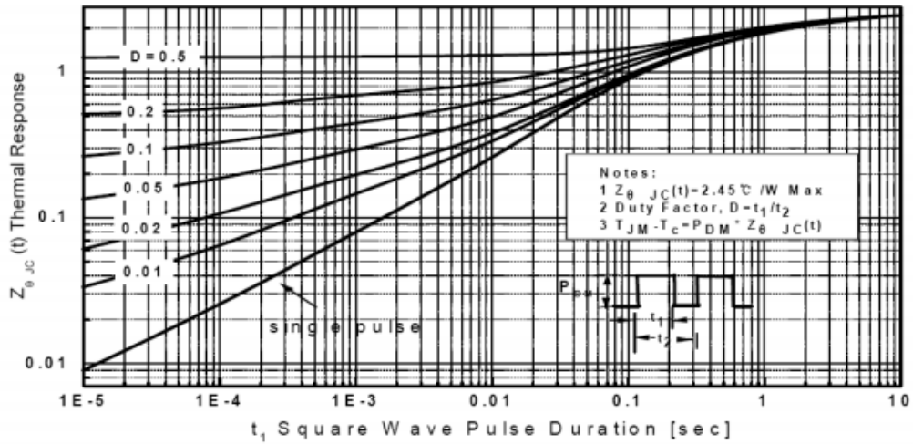
Transient Thermal Response Curve For TO-220F
