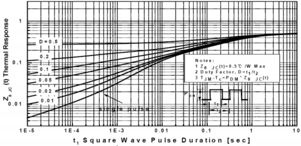
Transient Thermal Response Curve For TO-220/263/262
