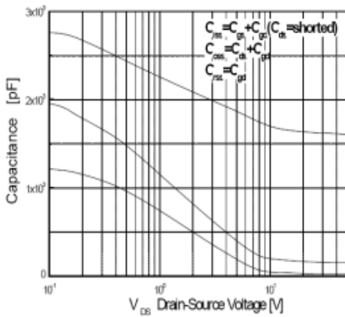
Capacitance Characteristics
