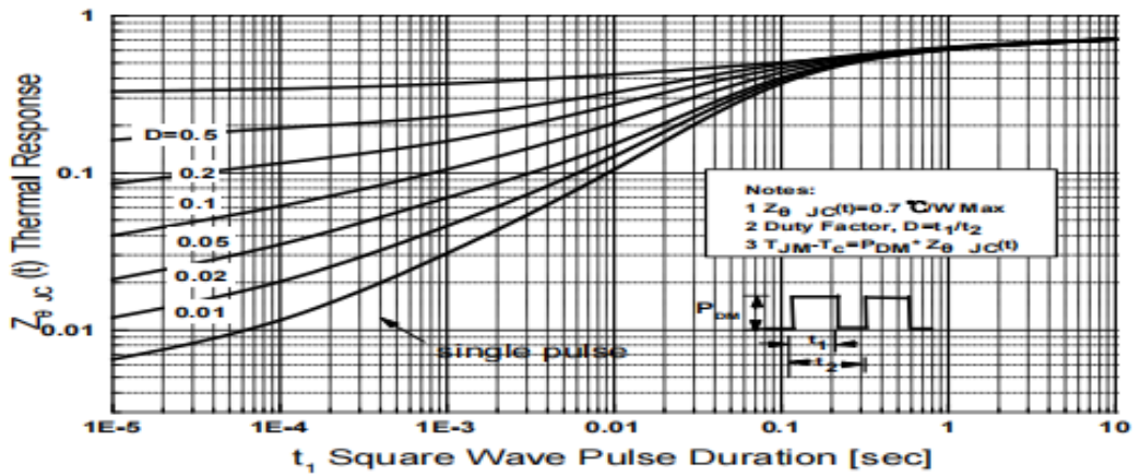
Transient Thermal Response Curve For TO-220/262/263
