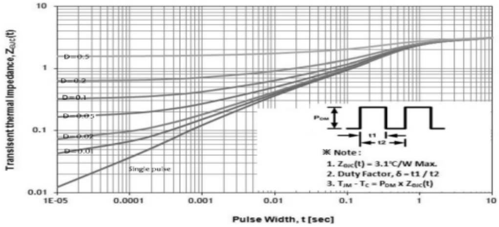
Transient Thermal Response Curve For TO-220F
