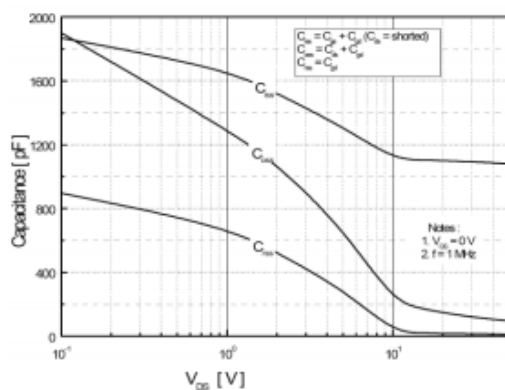
Capacitance Characteristics
