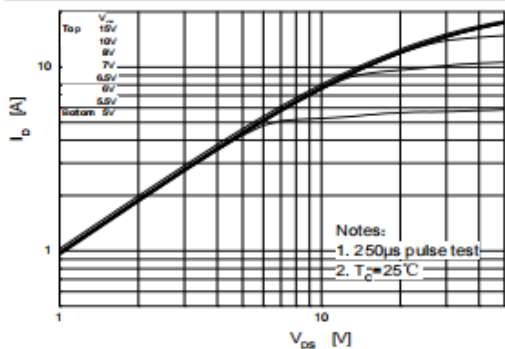
On-Region Characteristics
