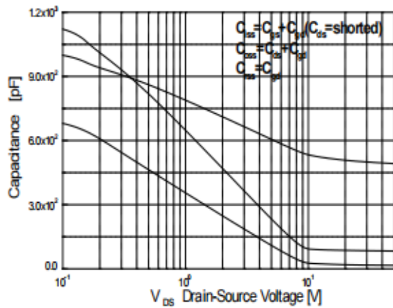
Capacitance Characteristics
