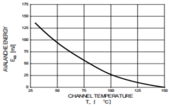
Avalanche Energy vs. Channel Temperature
