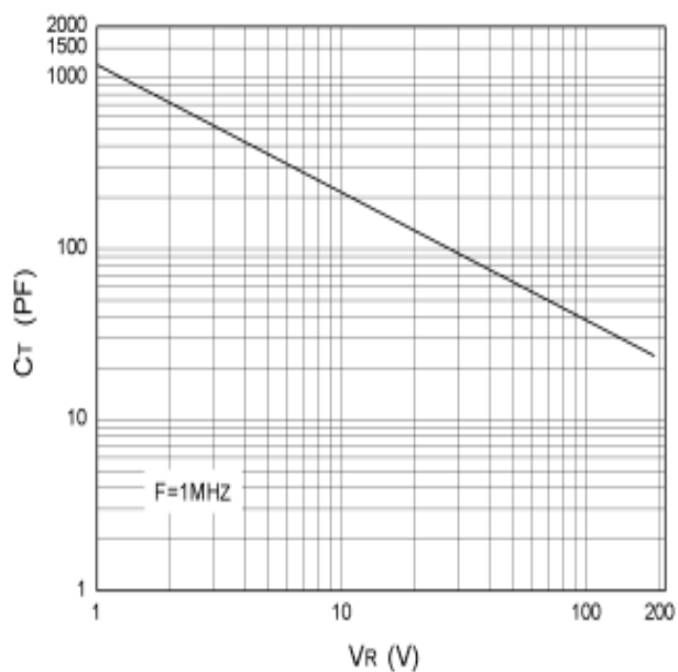
C_T vs V_R
