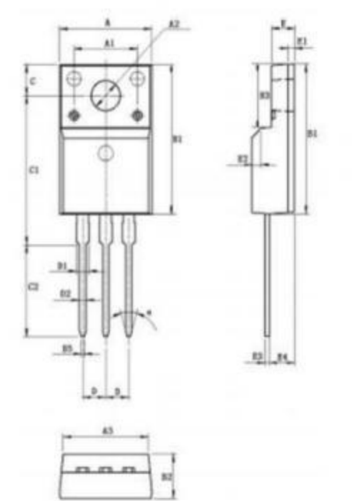
TO-220F
