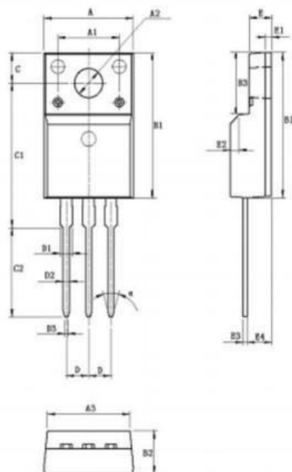
TO-220F
