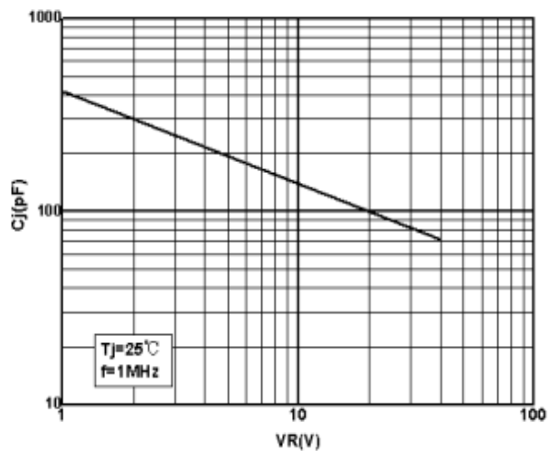
C_J vs V_R
